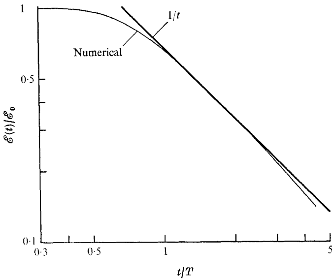
FIGURE 5. Decay of turbulent energy.
